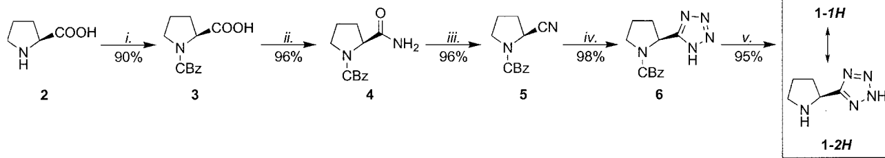
Scheme 2. Synthesis of 1 . (i) Cbz-Cl, NaOH, 5°C; (ii) (Boc) 2 O, NH 4 HCO 3 , CH 3 CN, cat. pyridine; (iii) Cyanuric chloride, DMF; (iv) NaN 3 , ZnBr 2 , water/2-propanol; (v) H 2 O, AcOH, H 2 , Pd/C.
