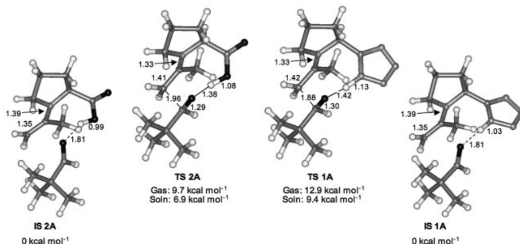
Figure 3. Geometry-optimized structures of the initial state and transition state of the proline (IS2A and TS2A) and tetrazole-catalyzed (IS1A and TS1A) asymmetric aldol reaction between acetone and 2,2-dimethylpropionaldehyde. Geometries are optimized at B3LYP/6-31G(d,p) level of theory and ZPE corrected. Energies in solution refers to single point B3LYP/6-311+G(d,p) calculations in DMSO using a self-consistent reaction field method and are ZPE corrected.
