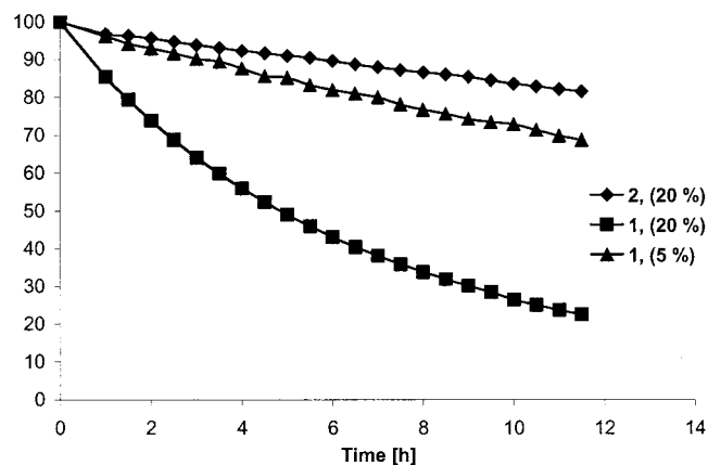
Figure 2. Graph showing the conversion of 2,2-dimethylpropionaldehyde ( 8 ) into the product ( R )-4-hydroxy-5,5-dimethylhexane-2-one as a function of time during the organocatalyzed direct asymmetric aldol reaction with acetone using catalyst 1 (20 mol%, and 5 mol%) and 2 (20 mol%).
