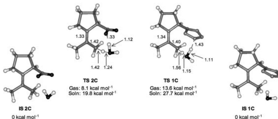
Figure 5. Geometry-optimized structures of the initial state and transition state of the proline- ( IS2C and TS2C ) and tetrazole-mediated ( IS1C and TS1C ) enamine formation occurring through the active participation of one water molecule. Geometries are optimized at B3LYP/6-31G(d,p) level of theory and ZPE corrected. Energies in solution refers to single point B3LYP/6-311+G(d,p) calculations in DMSO using a self-consistent reaction field method and are ZPE corrected.
