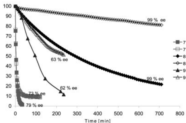
Figure 1. Graph showing the conversion of starting material into product as a function of time during the direct organocatalyzed asymmetric aldol reaction between acetone and aldehydes 4-nitrobenzaldehyde ( 7 ), 2,2-dimethylpropionaldehyde ( 8 ), and 4-methoxybenzaldehyde ( 9 ) using catalyst 1 (solid markers) and catalyst 2 (empty markers).
