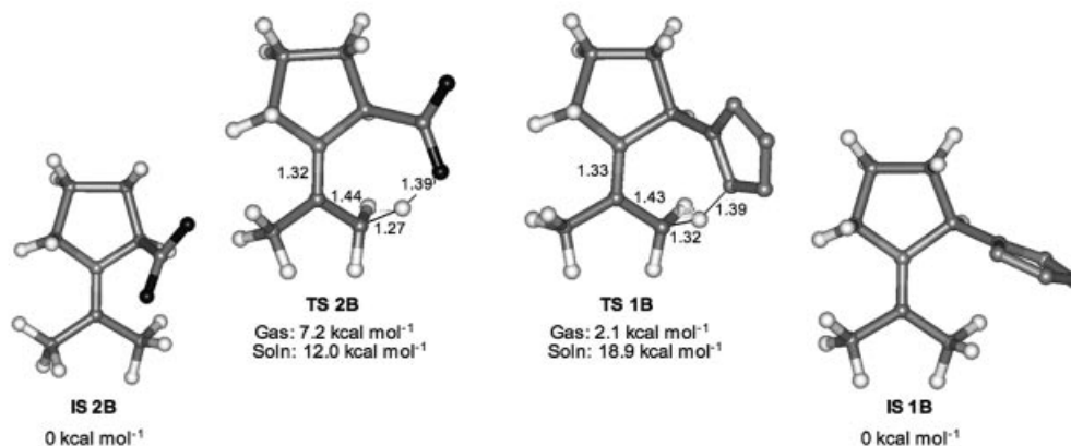
Figure 4. Geometry-optimized structures of the initial state and transition state of the proline ( IS2B and TS2B ) and tetrazole ( IS1B and TS1B ) mediated enamine formation. Geometries are optimized at B3LYP/6-31G(d,p) level of theory and ZPE corrected. Energies in solution refers to single point B3LYP/6-311+G(d,p) calculations in DMSO using a self-consistent reaction field method and are ZPE corrected.
