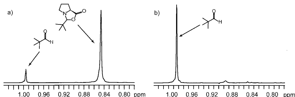
Figure 6. Expansion of ^1\text{H} NMR spectra of a mixture of 2,2-dimethylpropionaldehyde and 2 (a) or 1 (b) in [\text{D}_6]\text{DMSO} . The spectra show almost quantitative formation of bicyclic oxazolidinone with 2 while 1 does not take part in such equilibrium. Spectra recorded in [\text{D}_6]\text{DMSO} at C_{\text{cat.}} = 0.196 \text{ M} , C_{\text{aldehyde}} = 0.196 \text{ M} .
